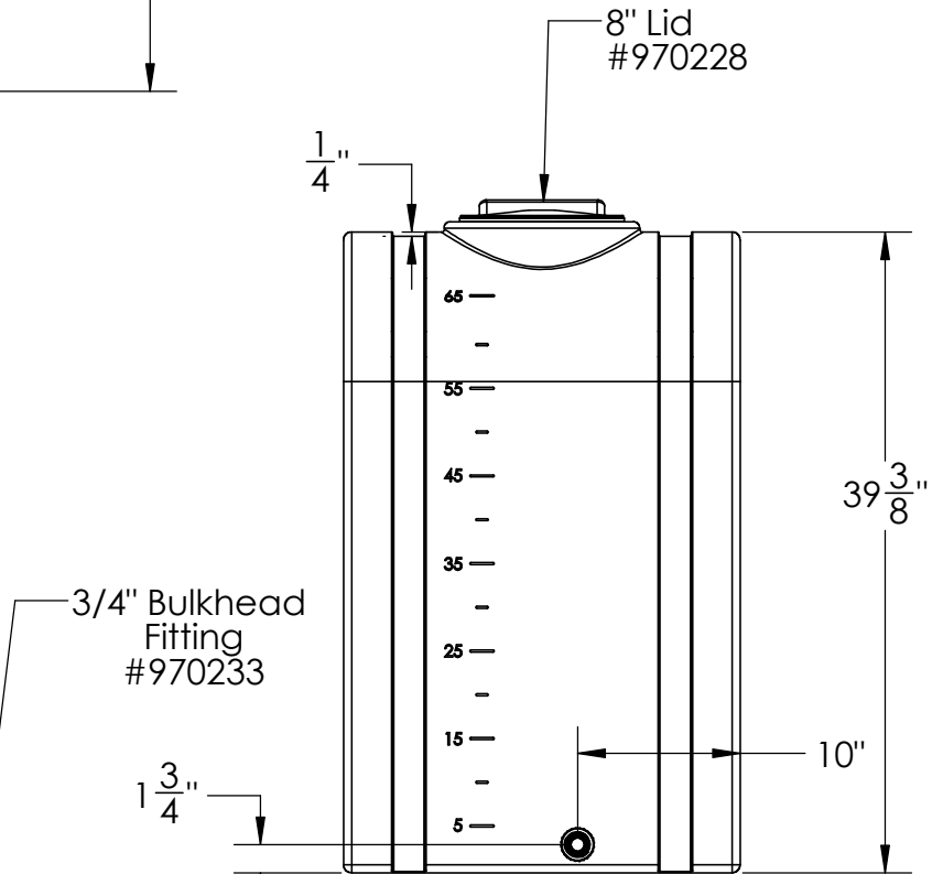
Natural 65 Gal Loaf Tank
